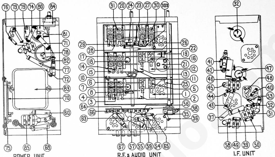
Fig. 3—Parts Locations—Underside View of Chassis.
