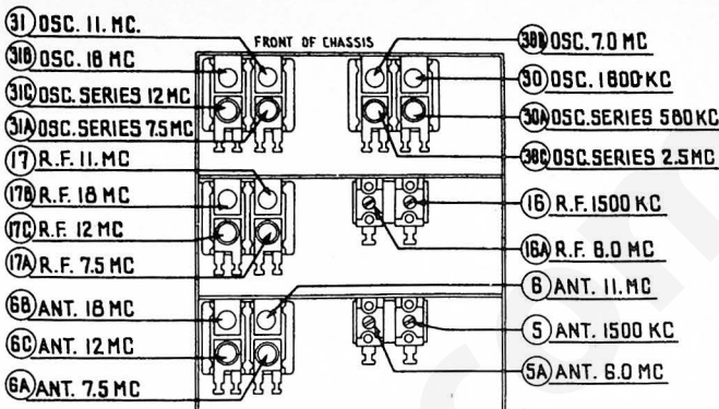
Fig. 6—Locations of R.F. Compensators Underside of Chassis
