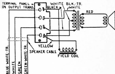
Speaker Wiring for Types K-36 and H-27
