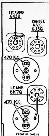
Fig. 5—Locations of I.F. Compensators Top of Chassis
